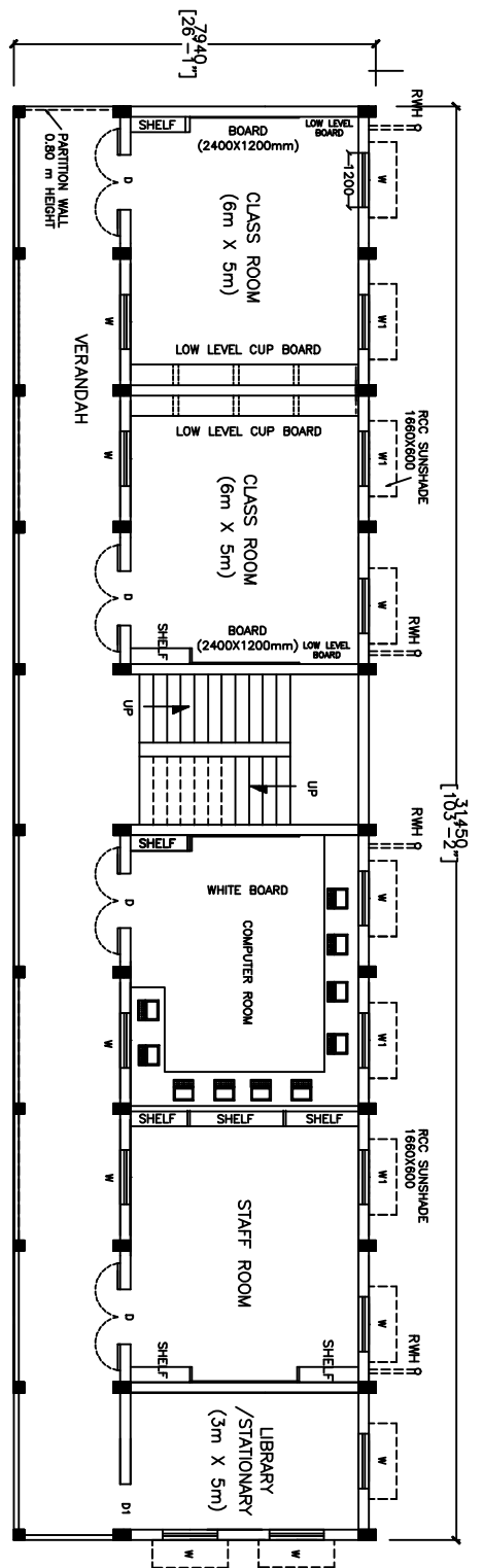
PLAN (FIRST FLOOR)
