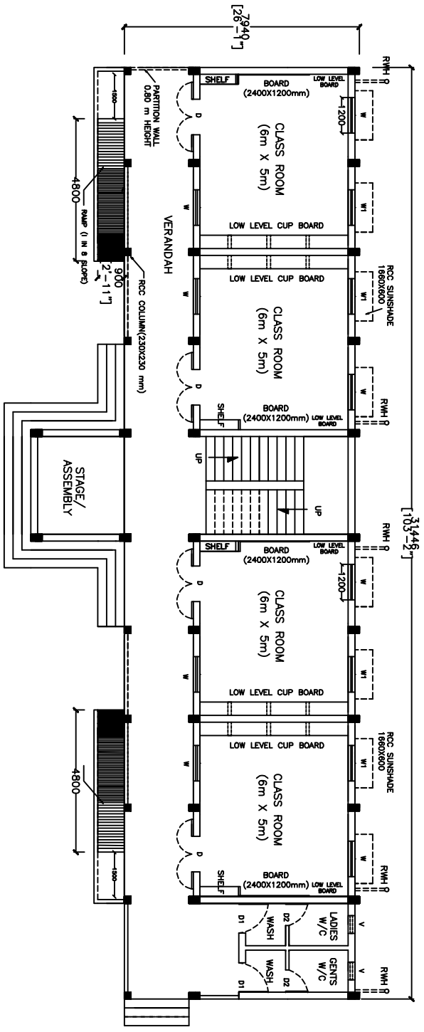
PLAN (FIRST FLOOR)
