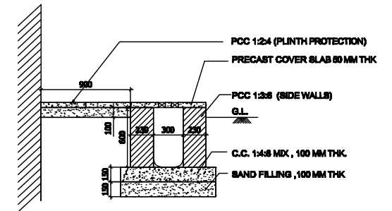
CROSS SECTION P - P PAVEMENT AND DRAIN
