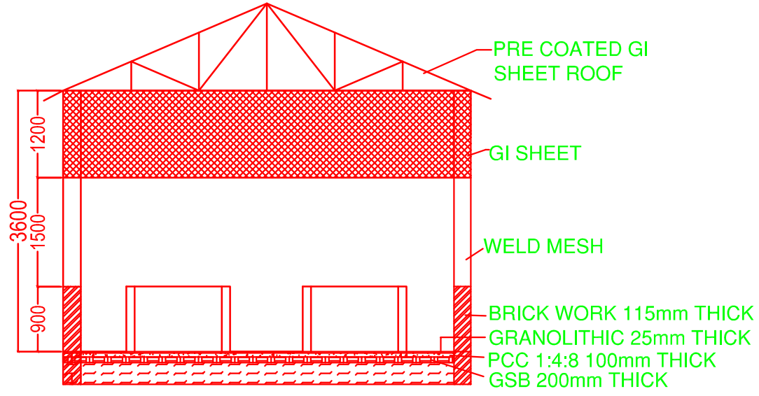
SECTION - SHED -WALL LOCATION
