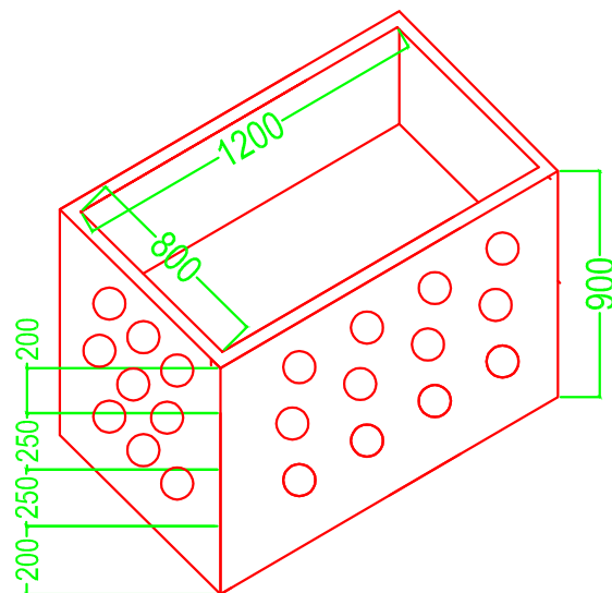
TUB SIDE PLAN
