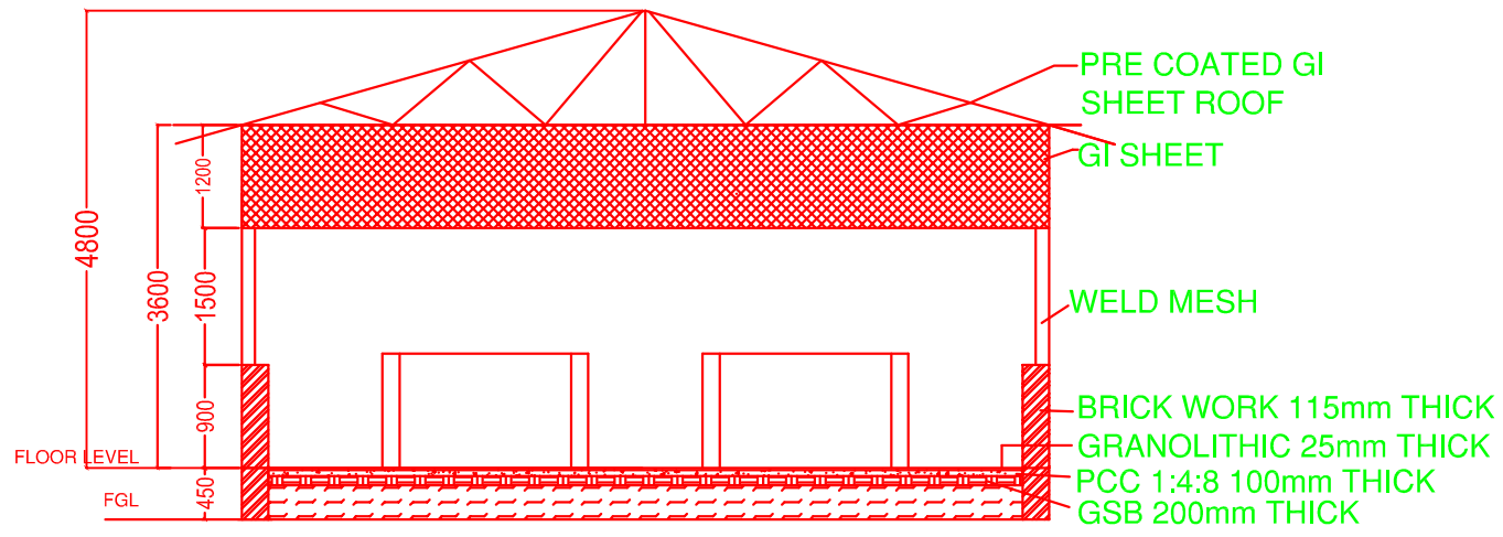
SECTION - SHED -WALL LOCATION
